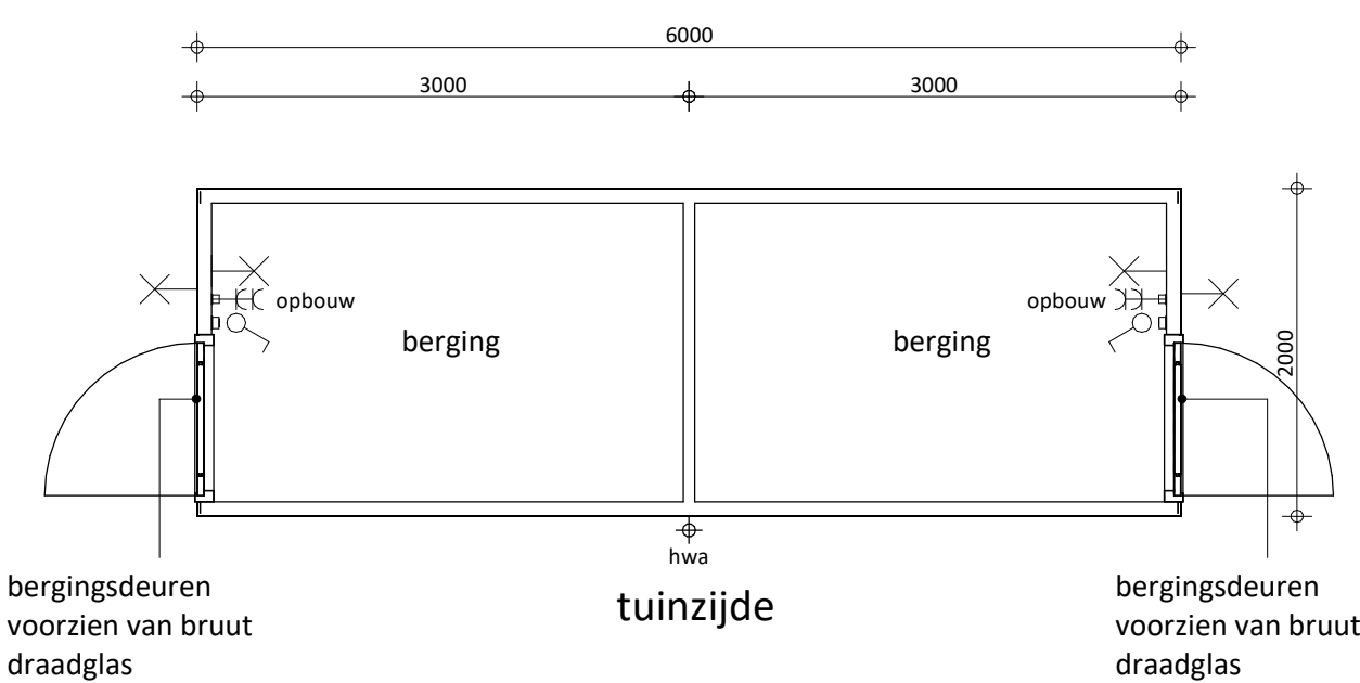
Plattegrond (type 2)
