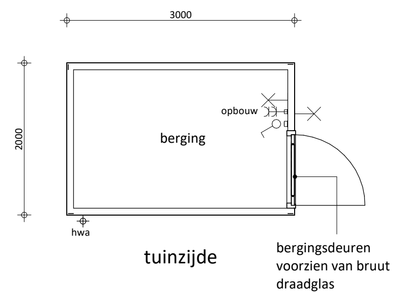
Plattegrond (type 1)
