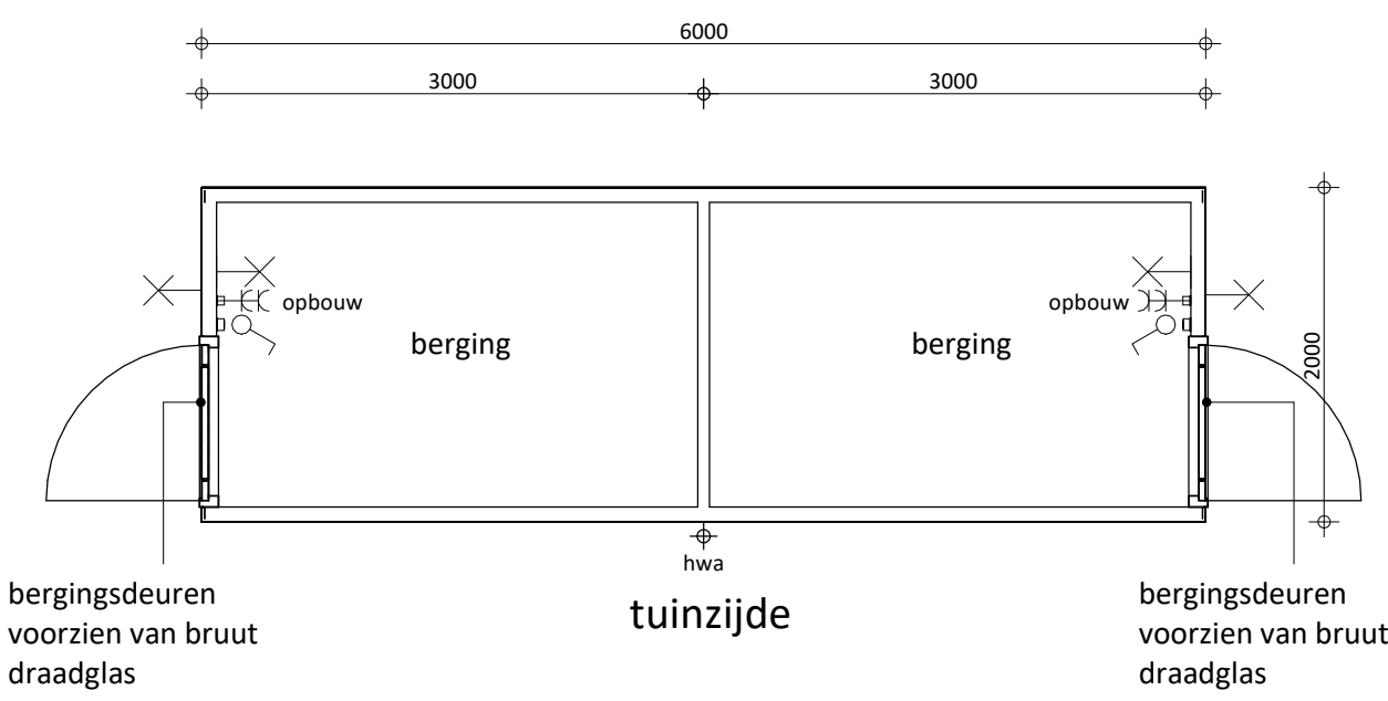
Plattegrond (type 2)
